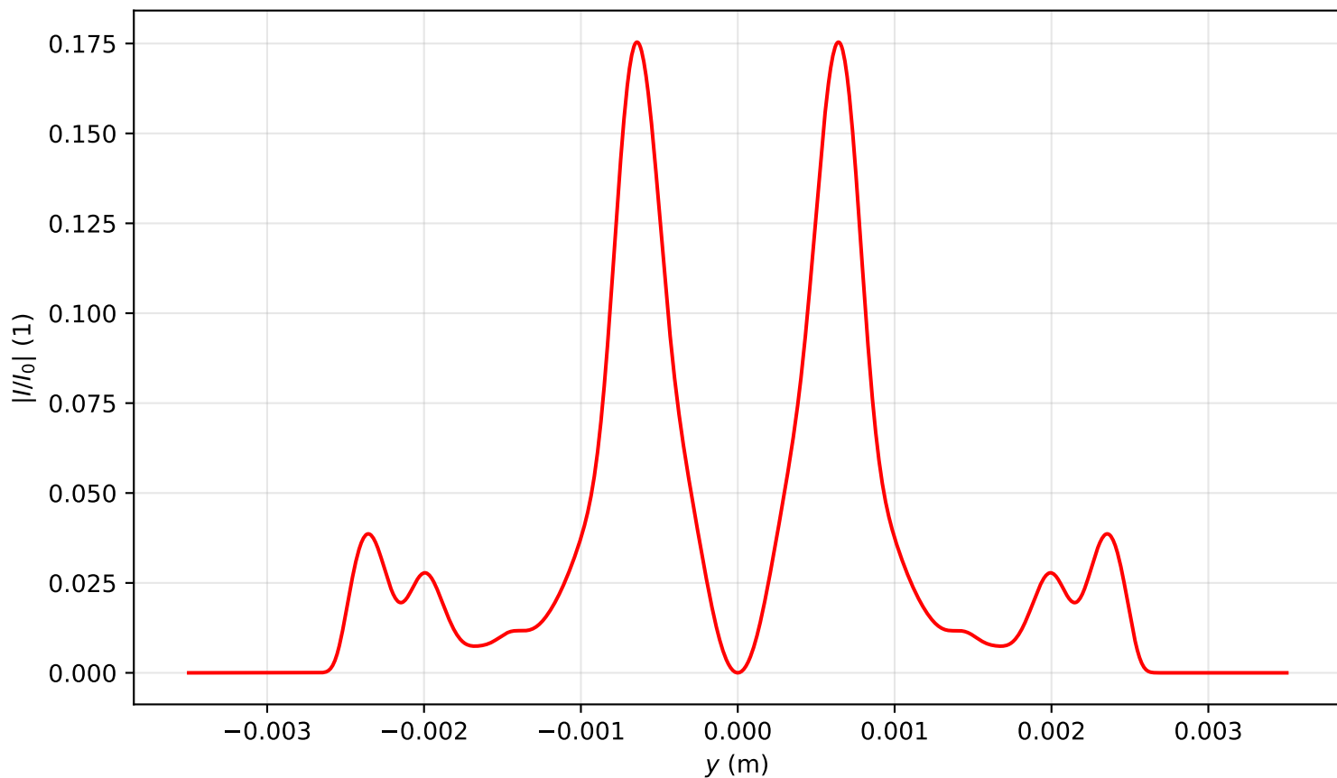
Intensity profile I(x=0, y, z=3.582)/I_0 , Pin=9.0Pcr, artificial time
